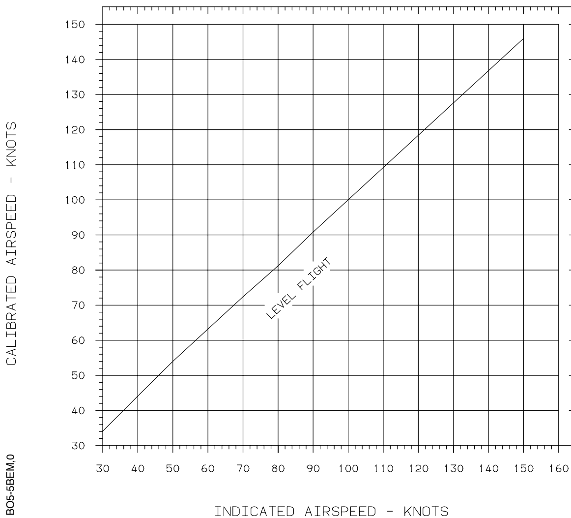
Fig. 5-4 Airspeed Calibration Chart
